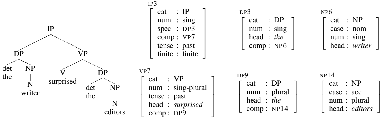
Figure 1. An example of chunks in ACT-R’s declarative memory, showing the chunk representation (right) of a syntactic structure (left).
