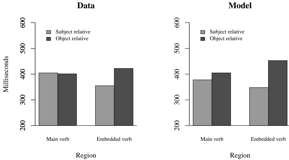
Figure 5. Model-generated and observed self-paced reading times on embedded verbs and main verbs in subject relative and object-relative clauses. Data from Experiment 1, Grodner & Gibson (2005).
