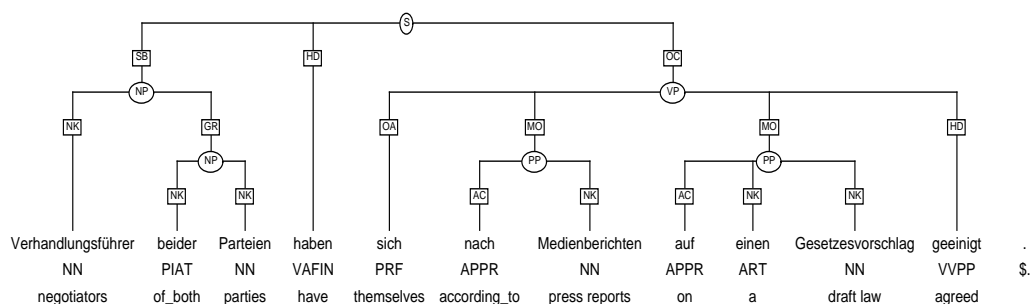
Figure 6: Annotation of PPs in NEGRA: MO
