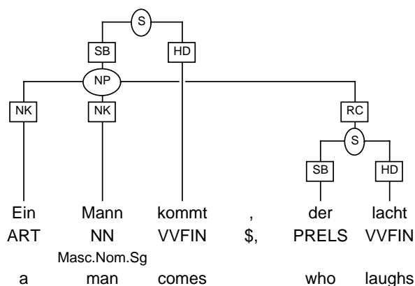
Figure 4: TIGER representation
