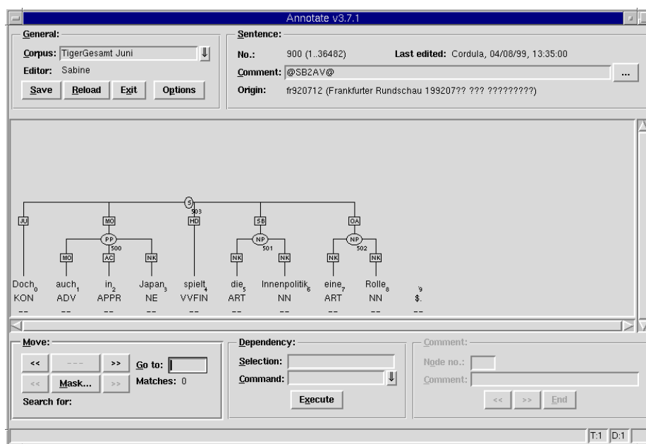
Figure 2: The annotation tool Annotate
