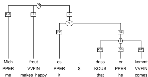
Figure 8: Correlative es
