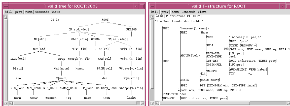
Figure 3: LFG c- and f-structure
