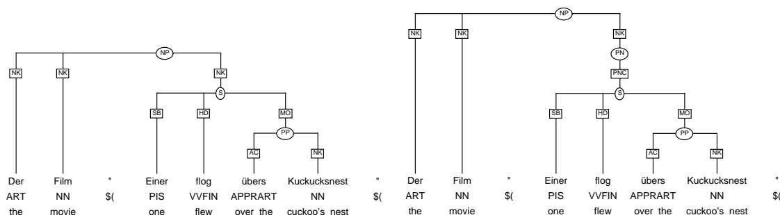
Figure 9: Treatment of structured proper nouns in NEGRA (left) and TIGER (right)
