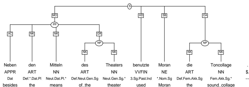
Figure 1: Different levels of annotation
