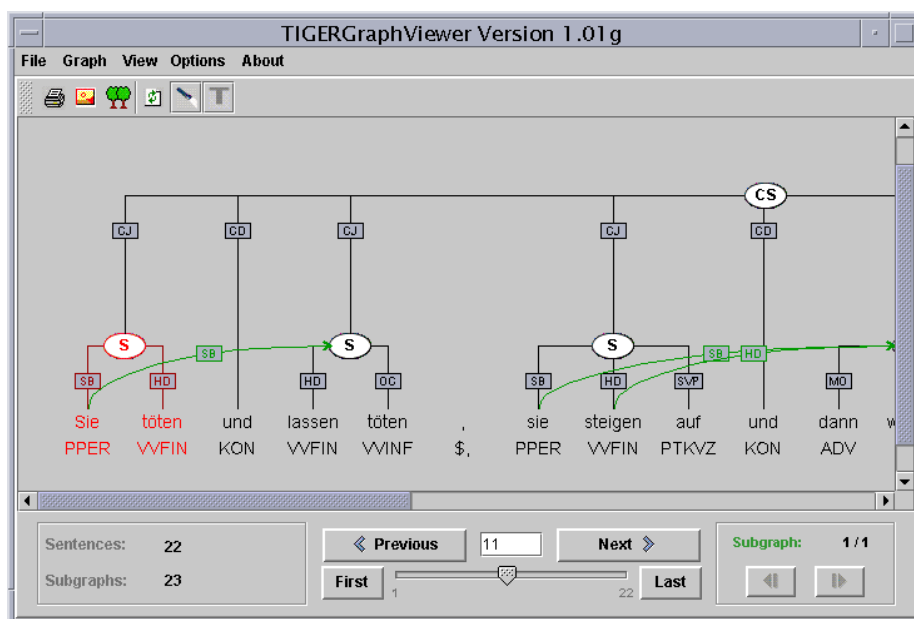
Figure 10: Visualization of query results
